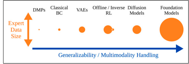
Figure 7. Reviewed learning approaches. Comparison of expert data requirements and ranking of generalization and multimodality handling capabilities. Offline and inverse RL approaches have similar generalization capacities. Inverse RL methods require much less expert data; however, they also require environment interactions.
